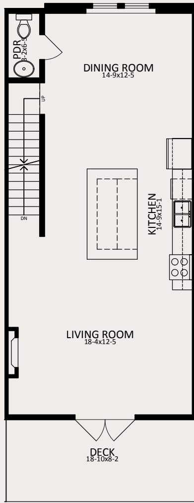
MAIN 792 sq. ft.
