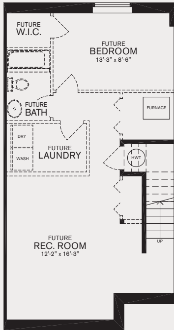
BASEMENT 710 SQ FT
